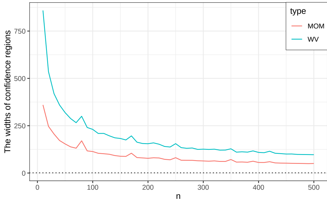
Standard Gaussian with 5% Pareto Noise
